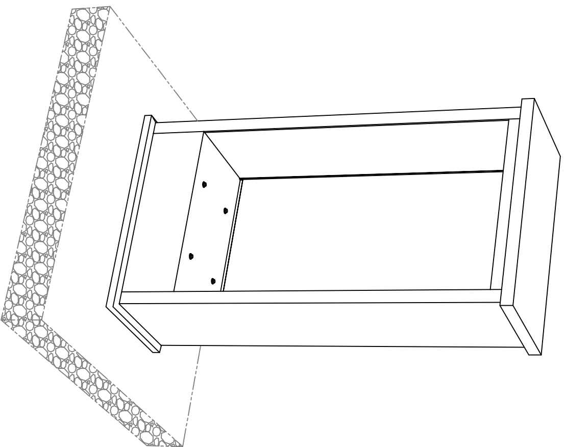
STEP 2b: Through the front opening, fasten four bolts to secure the kiosk to the base frame
