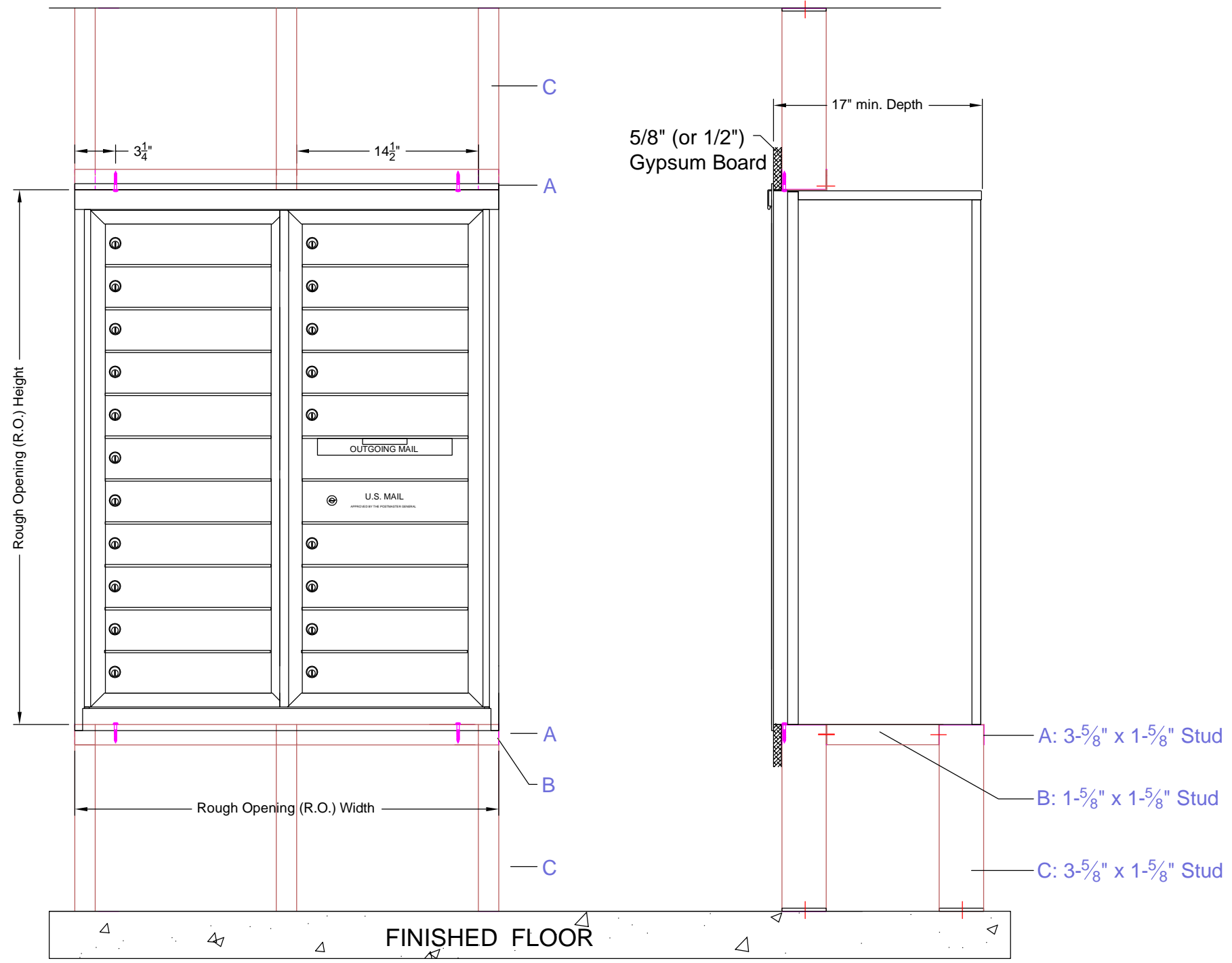
FRONT ELEVATION
